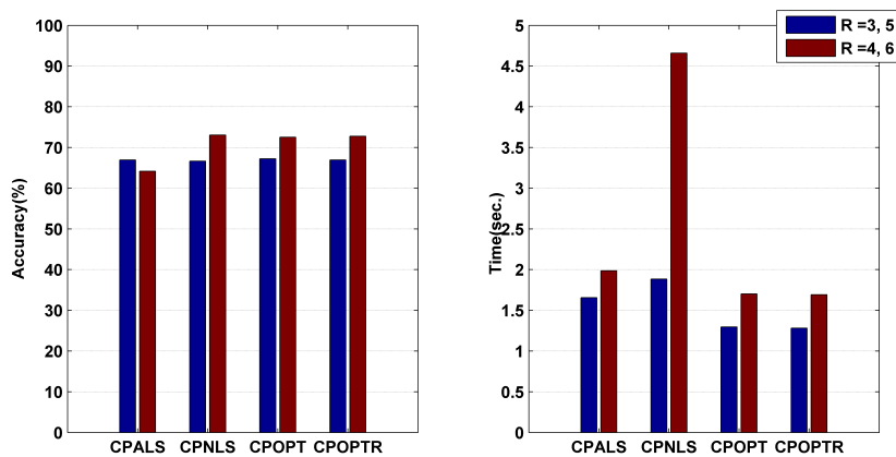
Fig. 6.4: Speed and accuracy comparison for computing the number of true underlying components (blue) and overfactoring (red) for tensors of size 50 \times 50 \times 50 and collinearity C = 0.9
